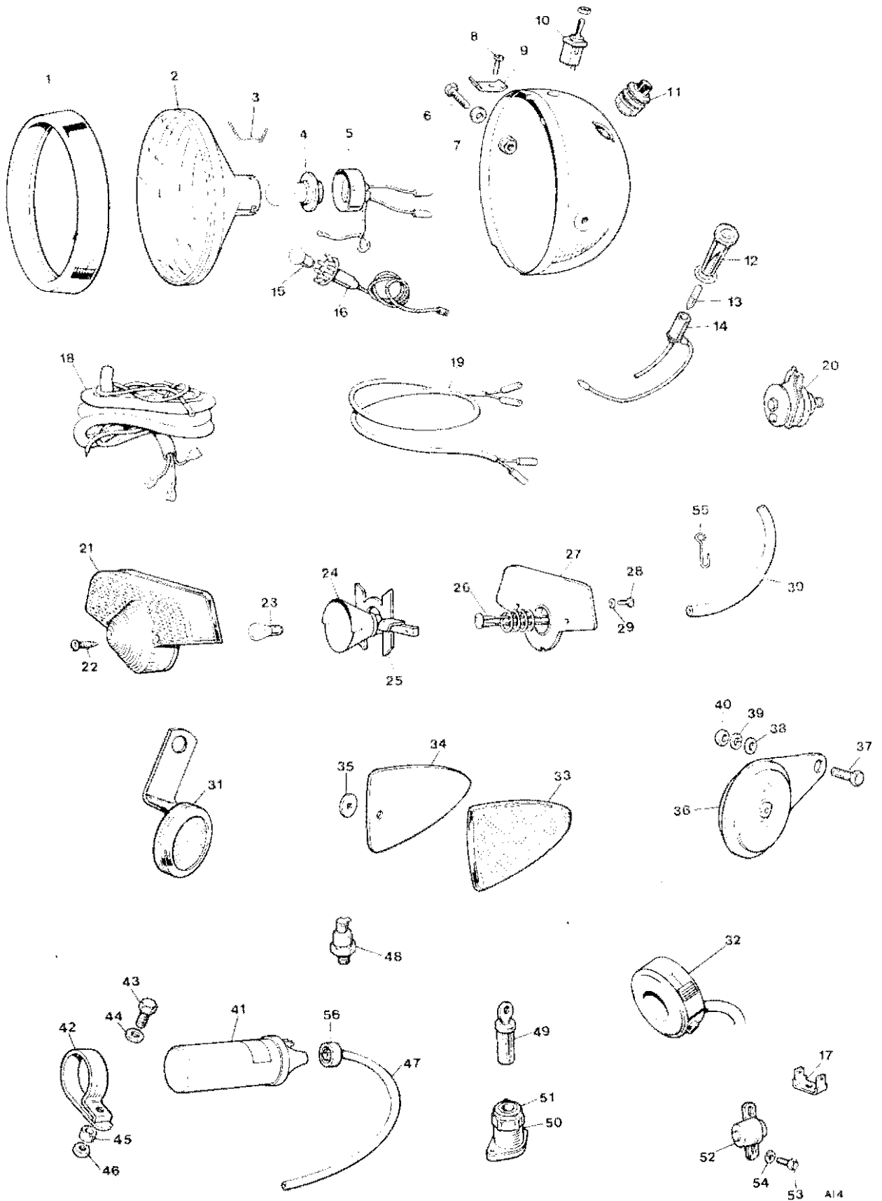
Fig. 16. ELECTRICAL EQUIPMENT
