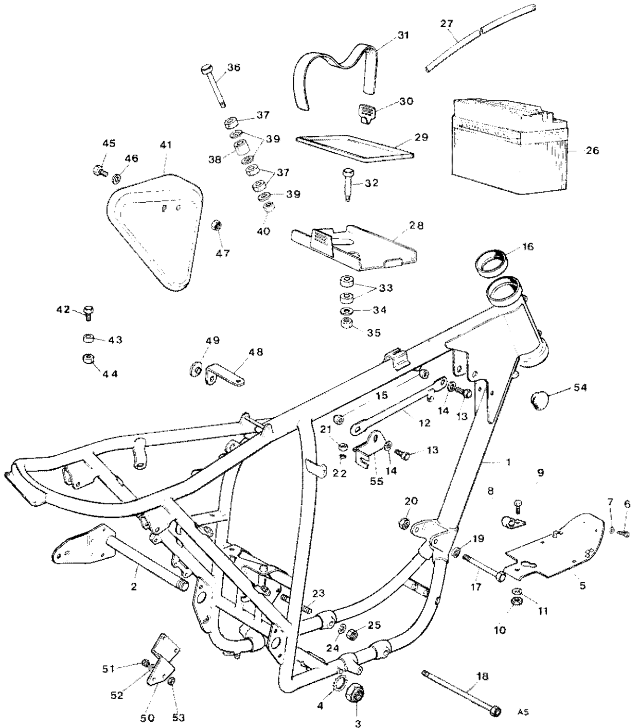
Fig. 5. FRAME COMPLETE
