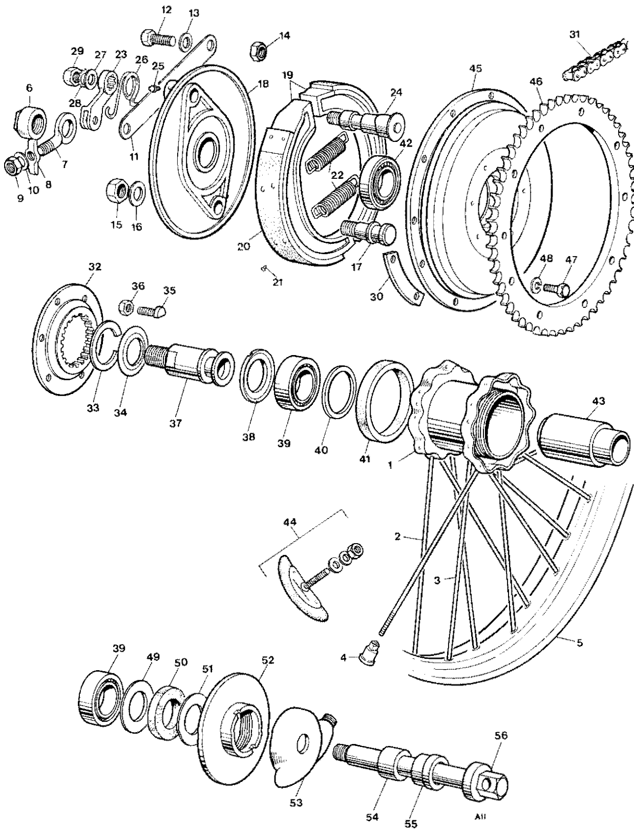
Fig. 11. REAR WHEEL
