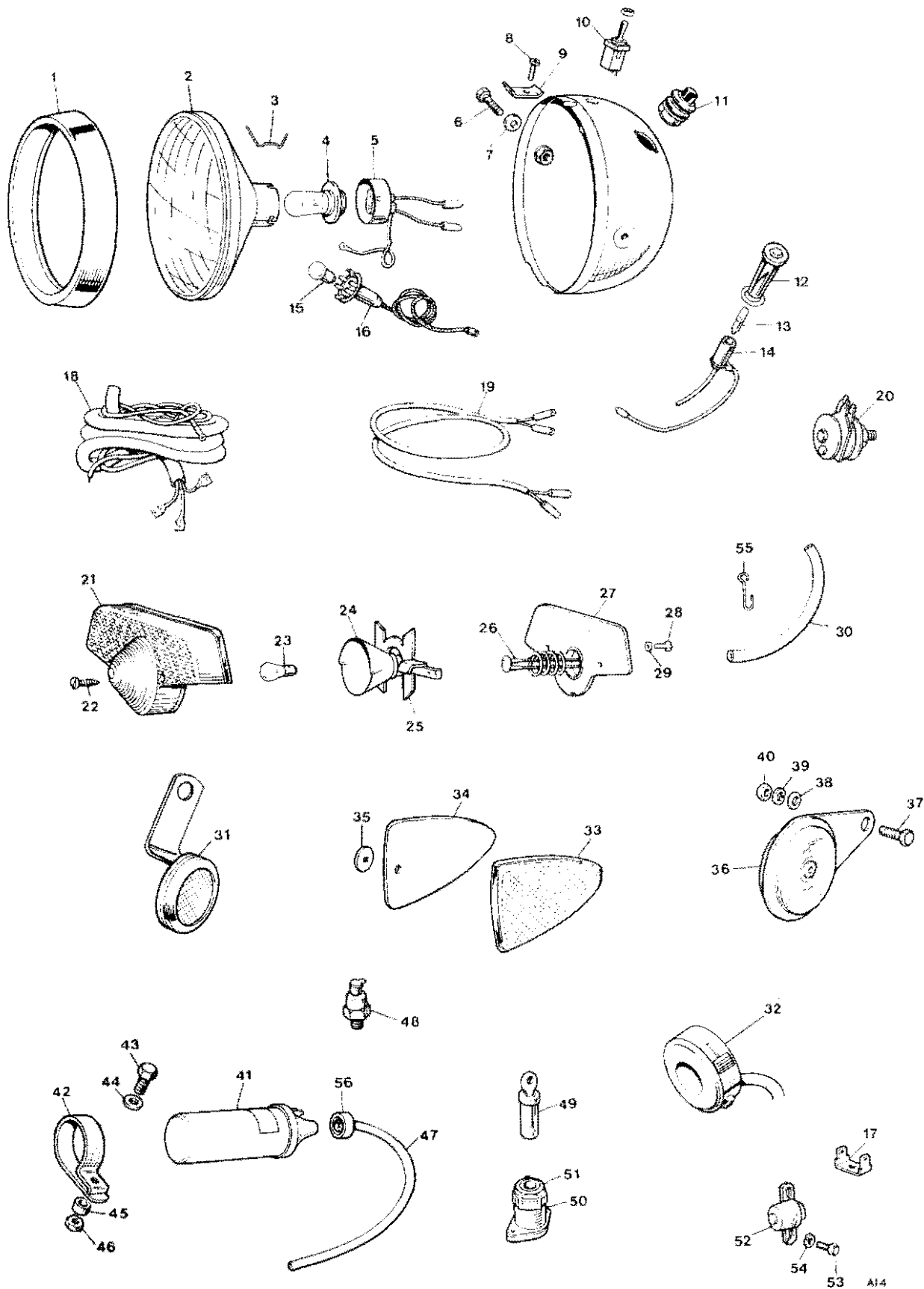
Fig. 16. ELECTRICAL EQUIPMENT
