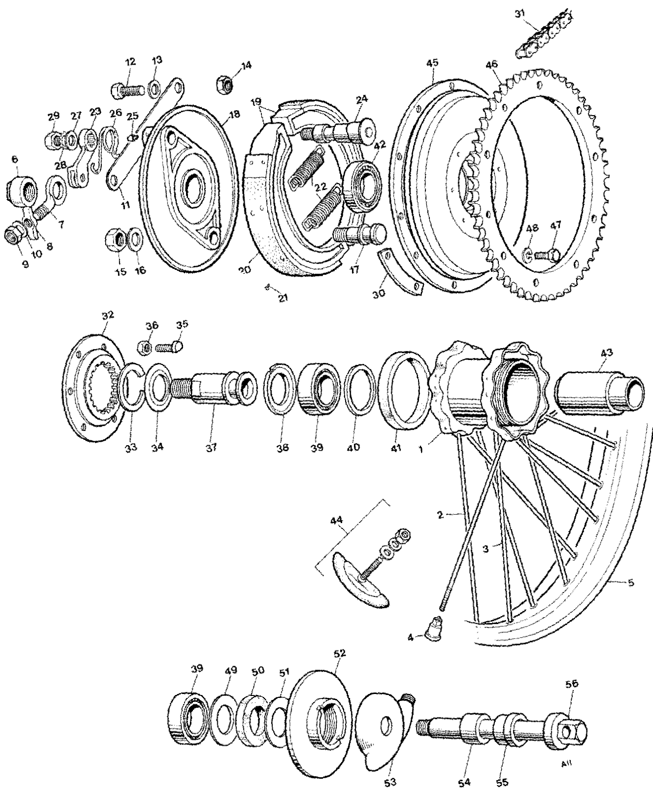
Fig. 11. REAR WHEEL
