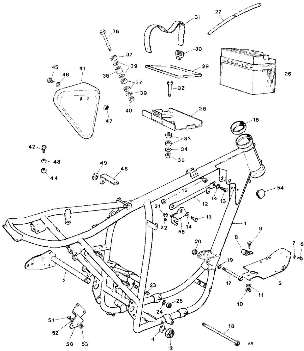
Fig. 5. FRAME COMPLETE
